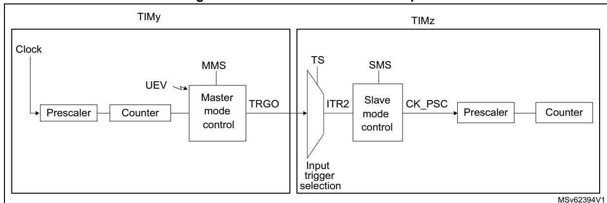
Figure 160. Master/Slave timer example
