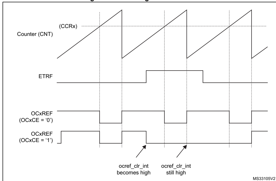
Figure 151. Clearing TIMx OCxREF
