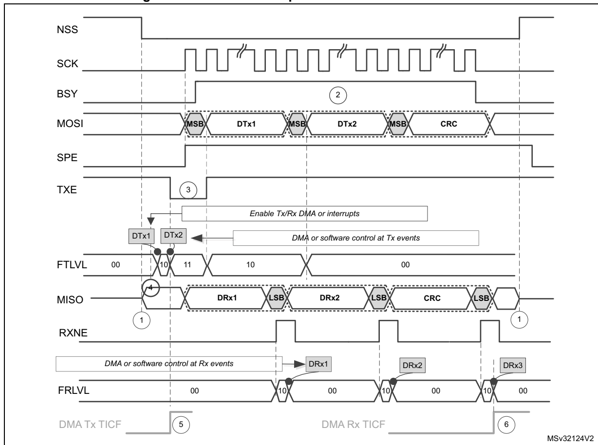
Figure 291. Master full-duplex communication with CRC
