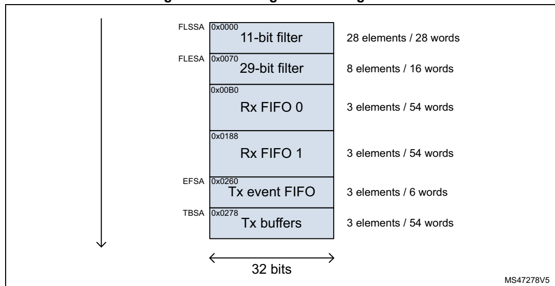
Figure 323. Message RAM configuration
