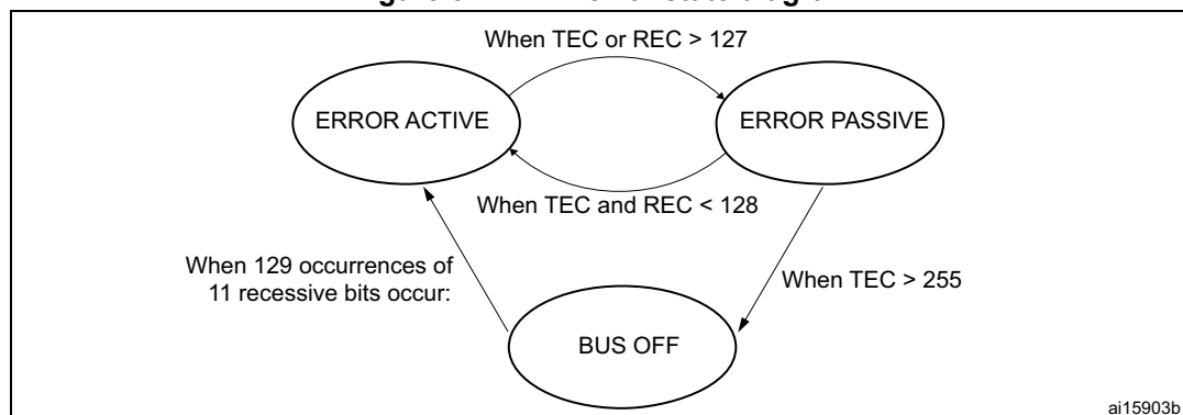
Figure 322. CAN error state diagram
