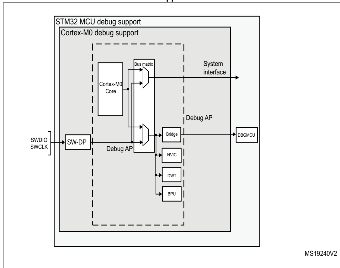
Figure 328. Block diagram of STM32C0 series MCU and Cortex ® -M0+-level debug support
