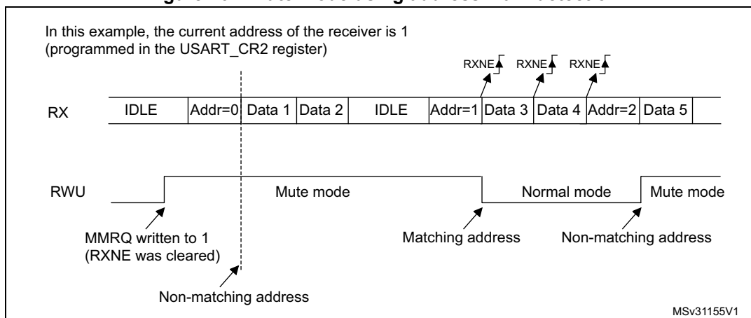
Figure 261. Mute mode using address mark detection
