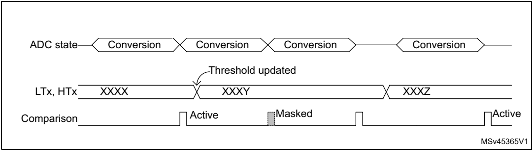
Figure 52. Analog watchdog threshold update
