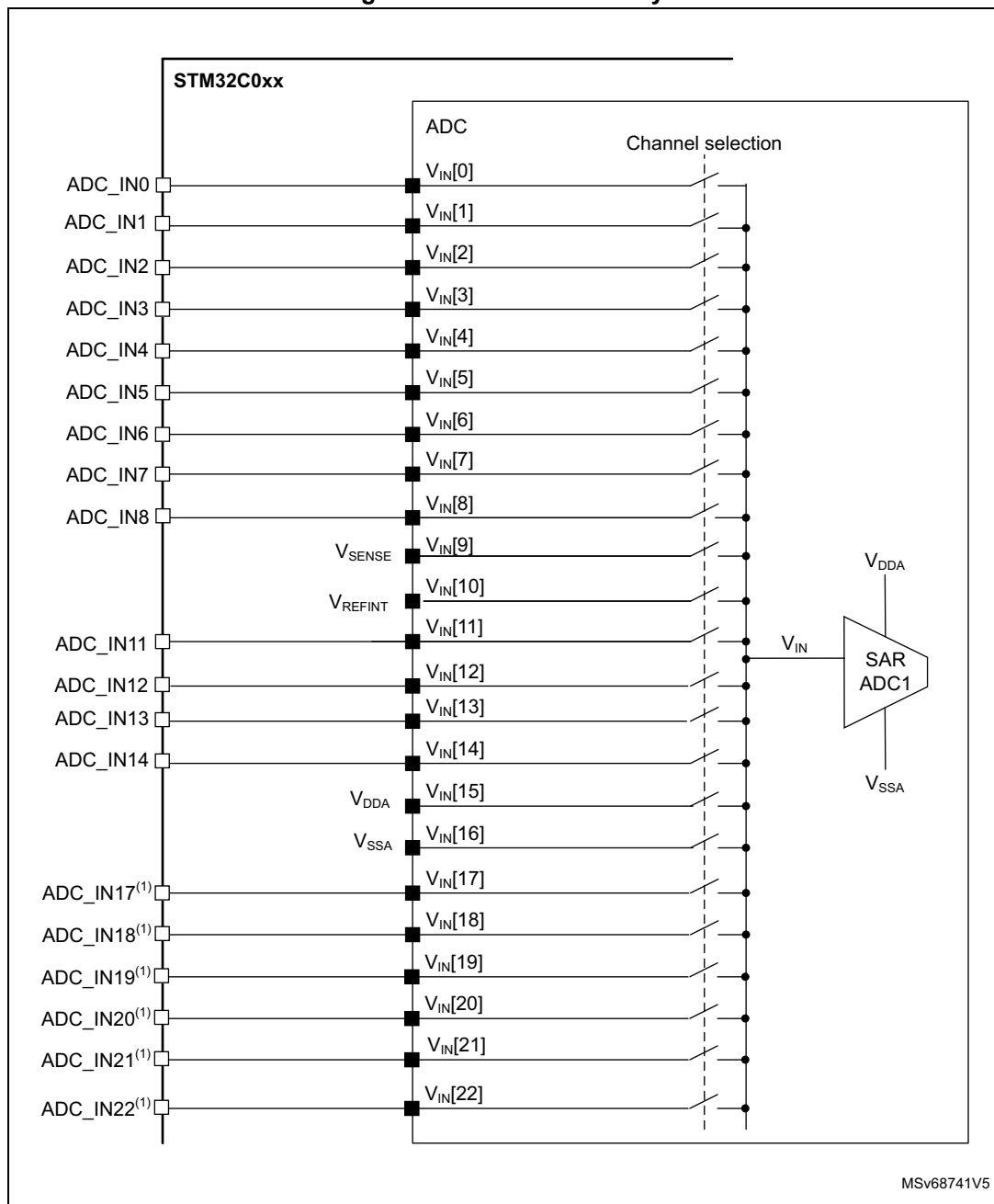
Figure 35. ADC connectivity
