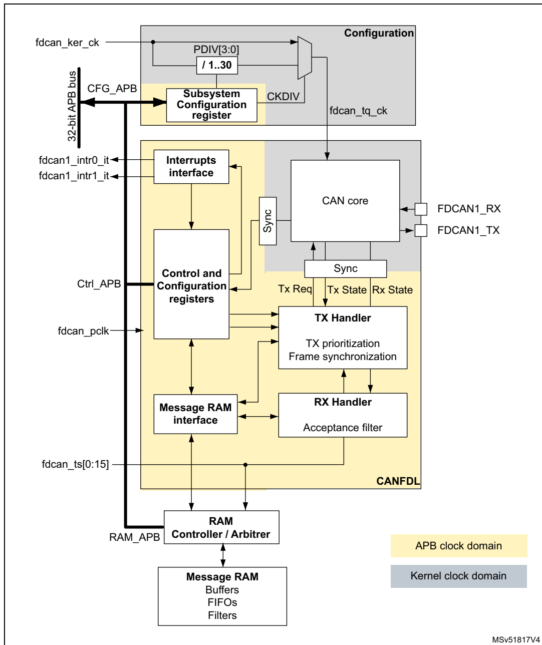
Figure 316. CAN subsystem.
