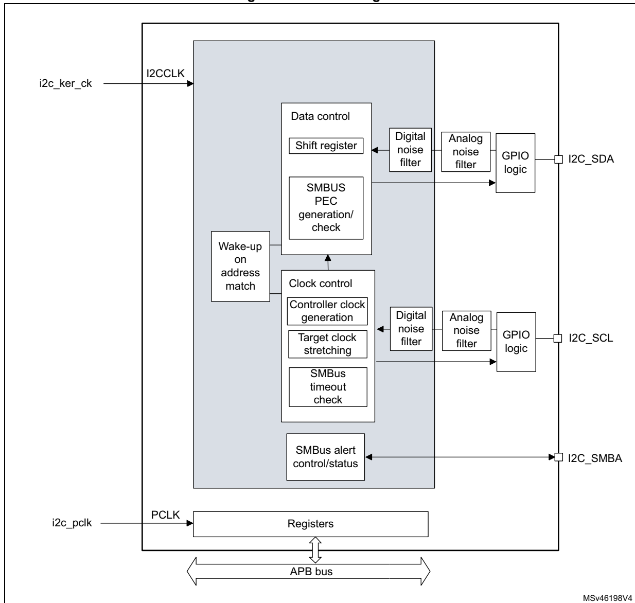
Figure 222. Block diagram
