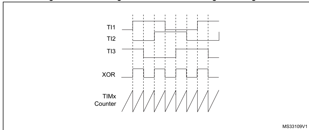
Figure 111. Measuring time interval between edges on 3 signals
