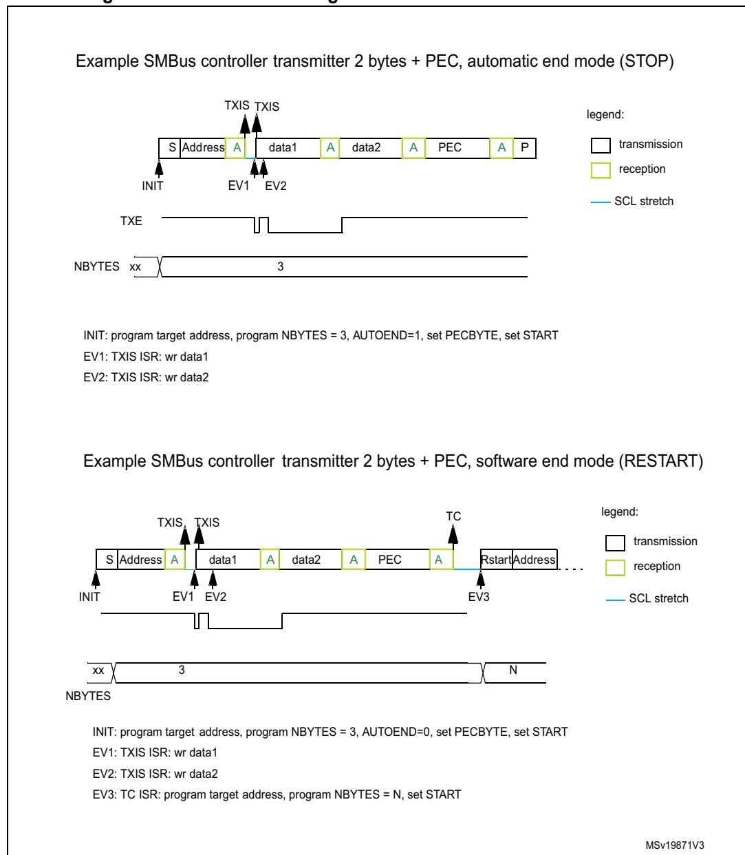
Figure 250. Bus transfer diagrams for SMBus controller transmitter
