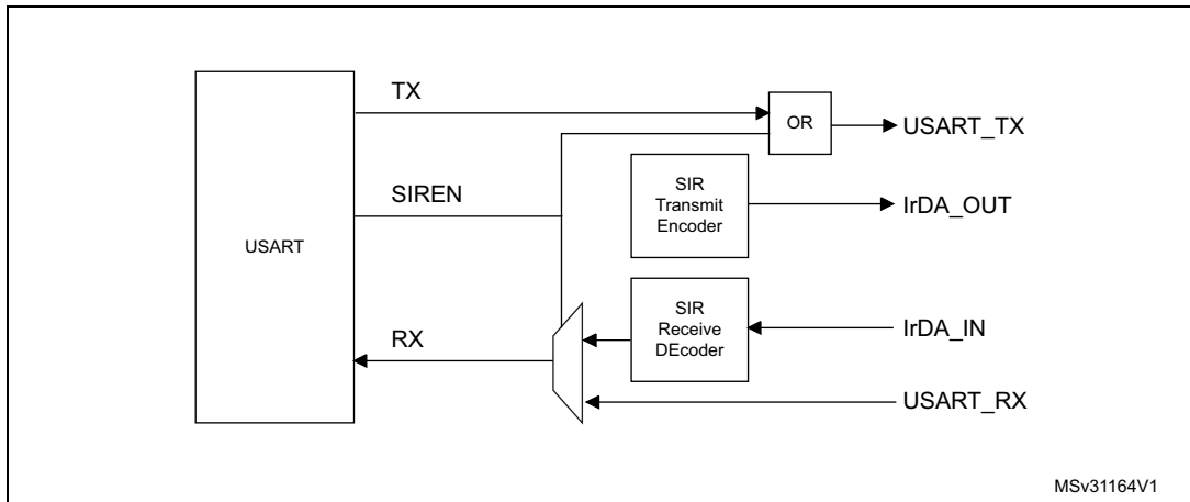
Figure 270. IrDA SIR ENDEC block diagram
