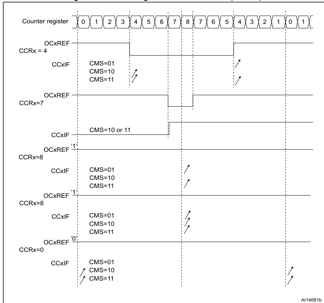
Figure 93. Center-aligned PWM waveforms (ARR=8)
