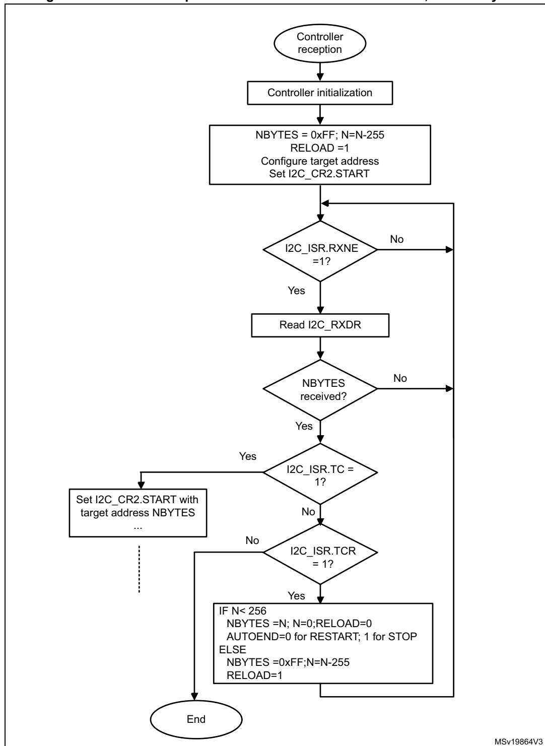
Figure 243. Transfer sequence flow for I2C controller receiver, N > 255 bytes
