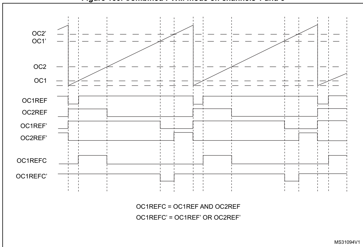
Figure 150. Combined PWM mode on channels 1 and 3
