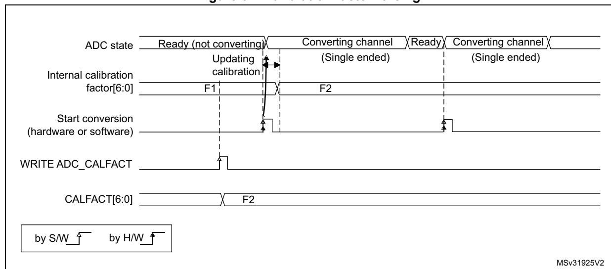
Figure 32. Calibration factor forcing
