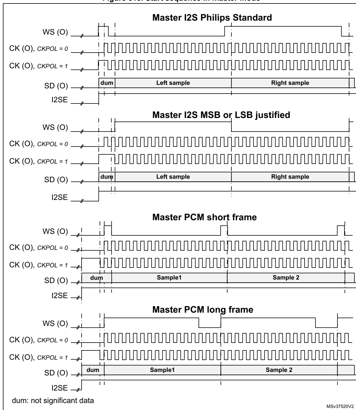
Figure 313. Start sequence in master mode
