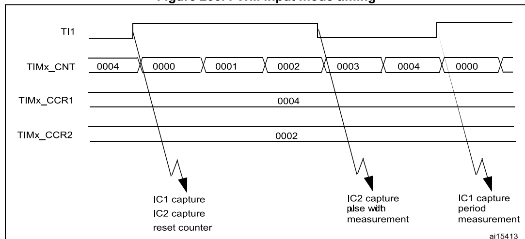
Figure 200. PWM input mode timing
