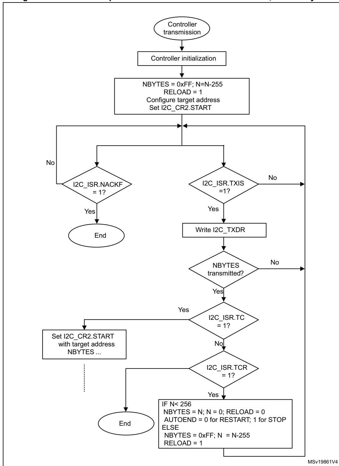
Figure 240. Transfer sequence flow for I2C controller transmitter, N > 255 bytes
