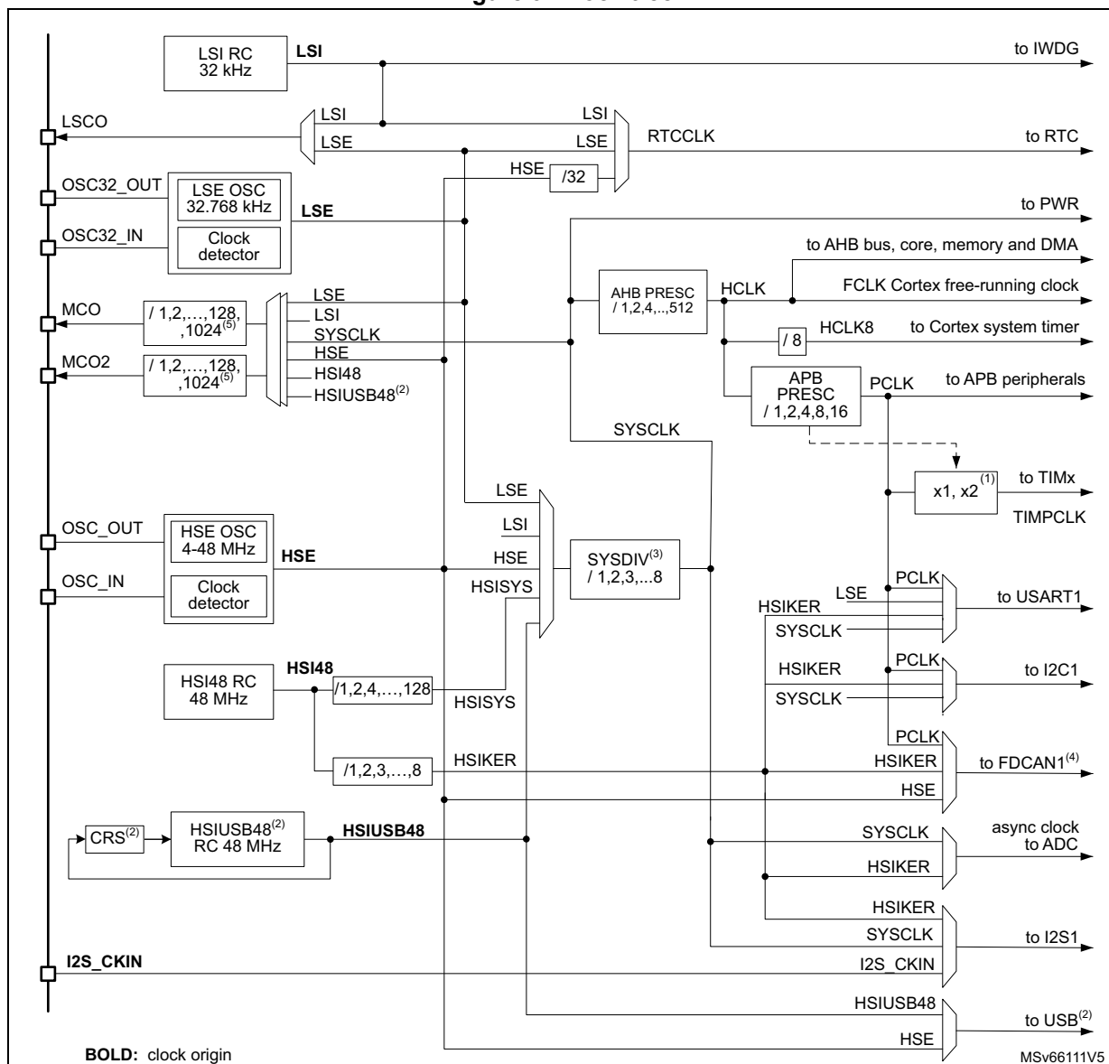
Figure 9. Clock tree
